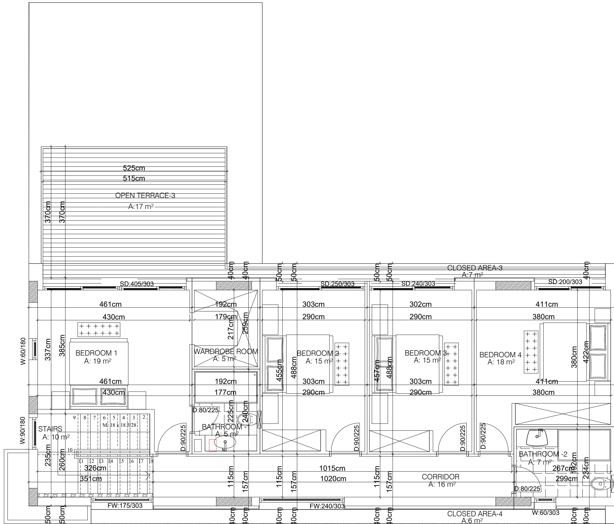
TYPE A- 1. FLOOR PLAN
